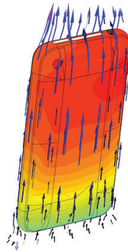
Figure 11. Case temperatures and buoyancy-driven airflow shown on a Simcenter Flotherm XT model of a Smartphone.
