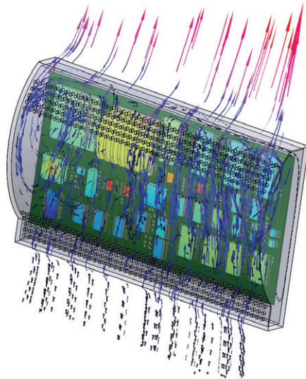
Figure 10. Flow distribution in Simcenter Flotherm XT showing the optimized vent arrangement for a naturally ventilated, wall mounted electronics system.
